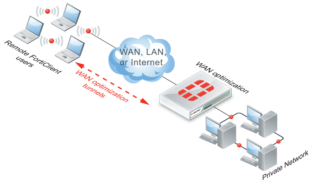
Figure 27: FortiClient WAN optimization topology
