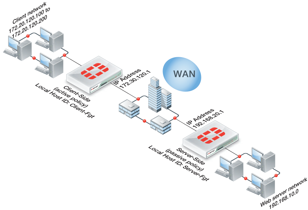
Figure 20: Example active-passive WAN optimization topology
