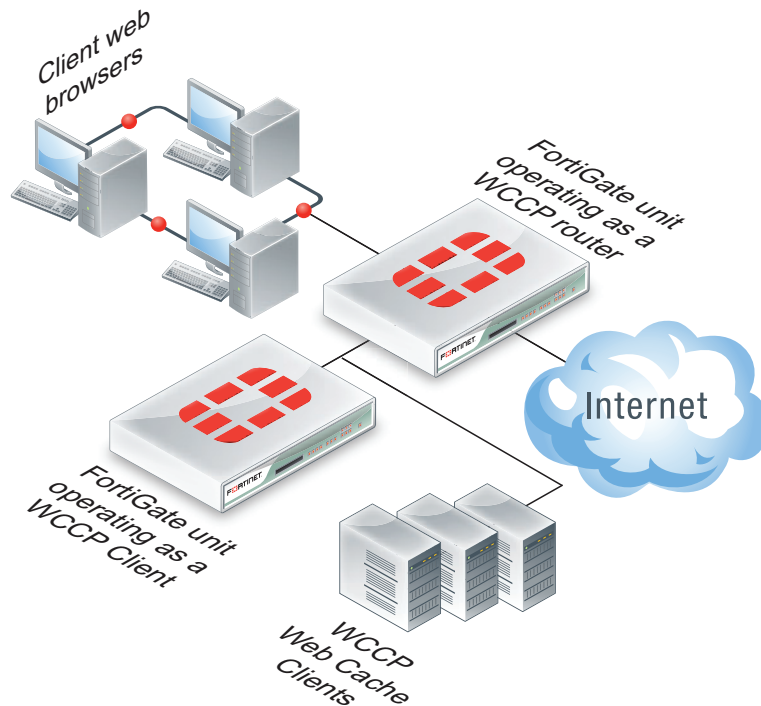
Figure 13: WCCP topology
