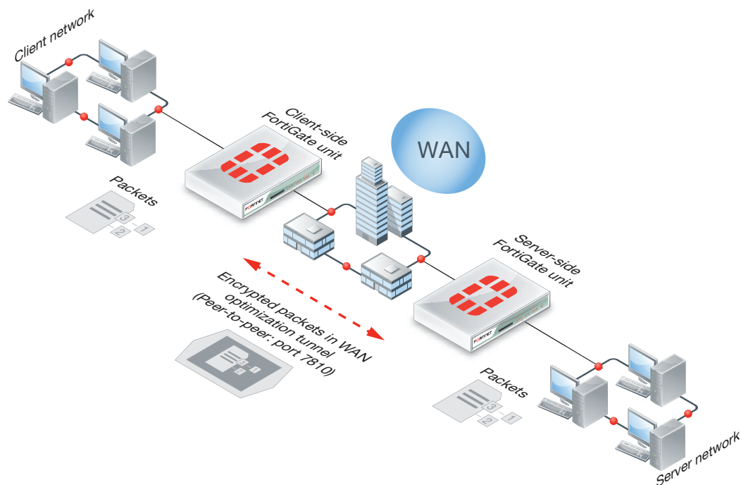
Figure 17: WAN optimization tunnels
