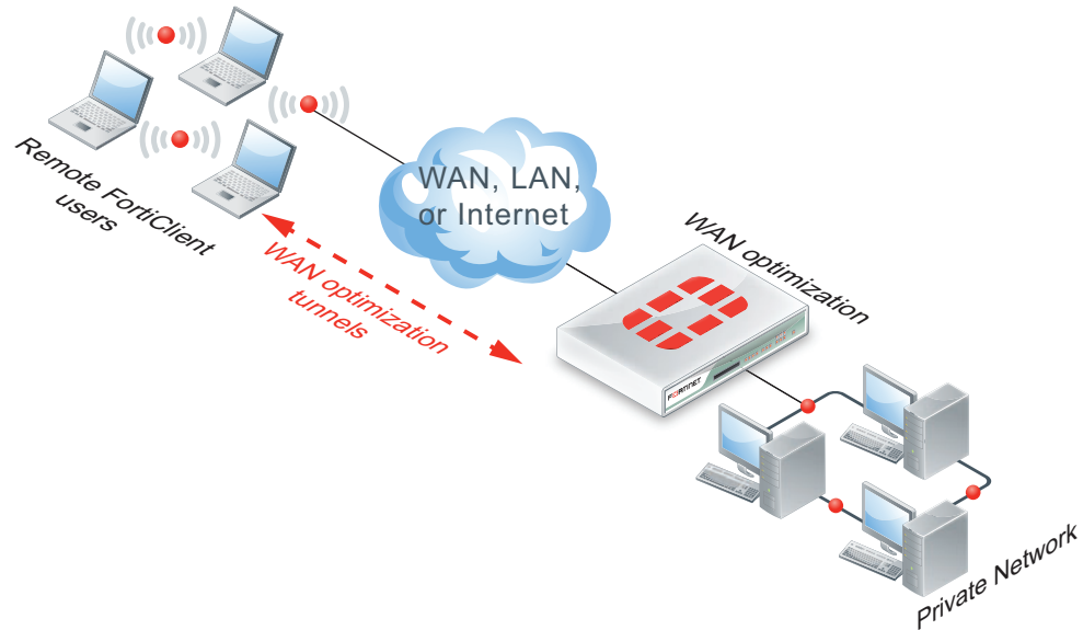
Figure 6: FortiClient WAN optimization topology
