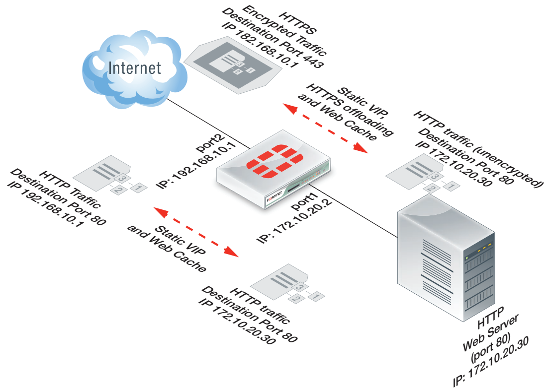
Figure 26: Reverse proxy web caching and SSL offloading for an Internet web server using static one-to-one virtual IPs
