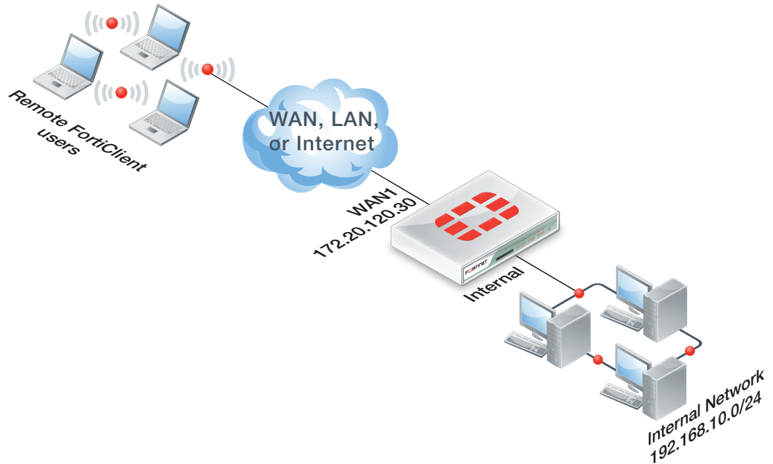
Figure 28: Example FortiClient WAN optimization configuration
