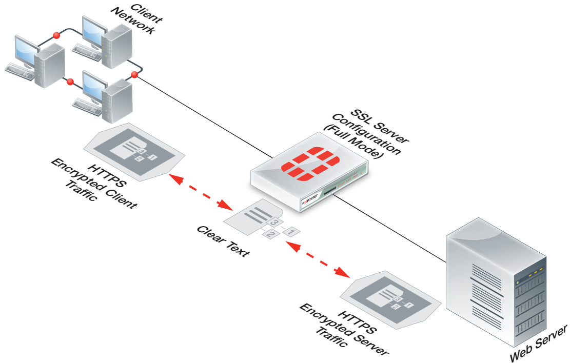
Figure 22: Full mode SSL server configuration
