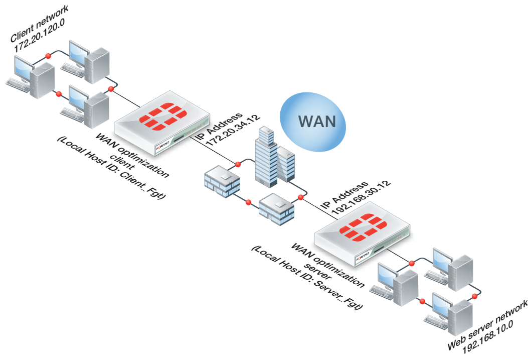
Figure 19: Example manual (peer-to-peer) topology
