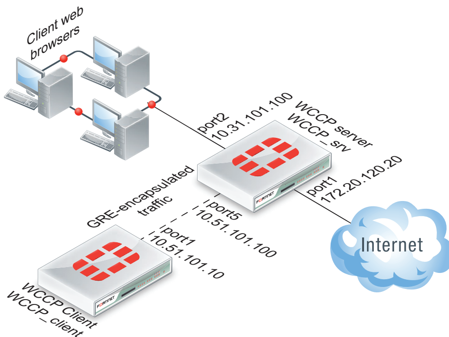
Figure 35: FortiGate WCCP server and client configuration
