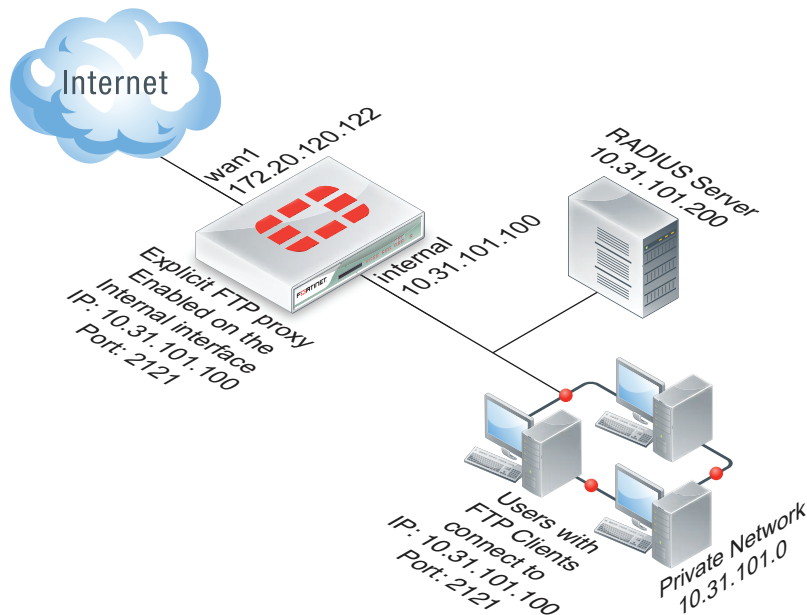
Figure 34: Example explicit FTP proxy network topology
